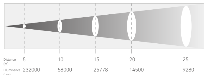
Beam Angle 52°
