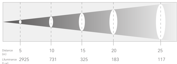
Beam Angle 52°
